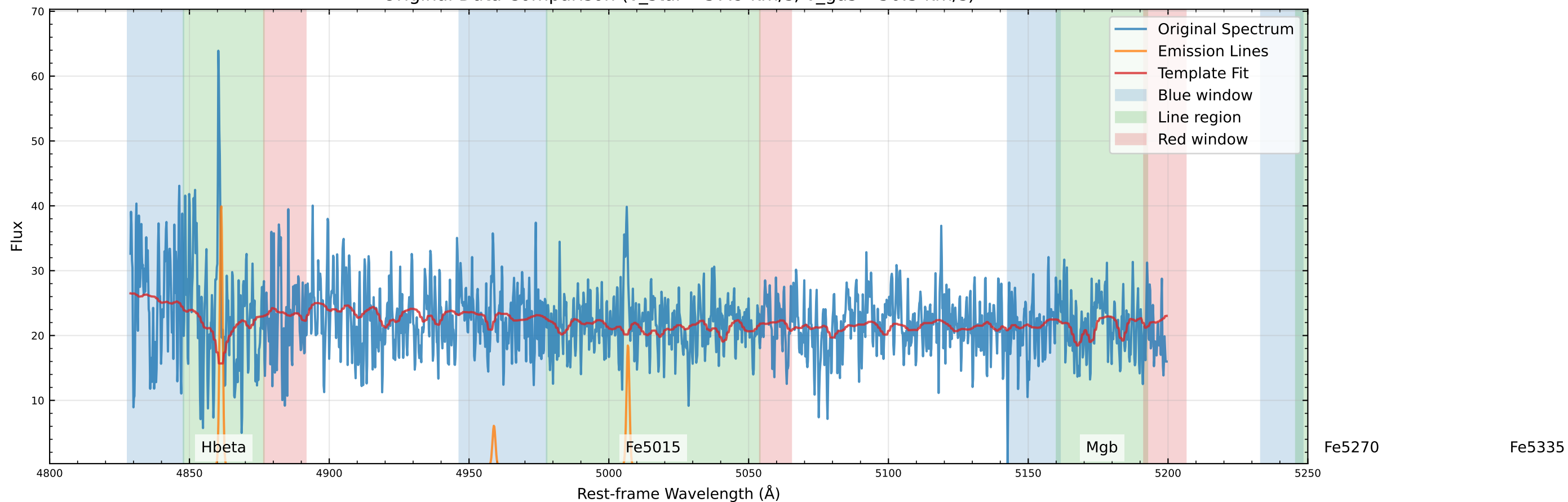
Original Data Comparison (v_star=-57.9 km/s, v_gas=-50.3 km/s)
