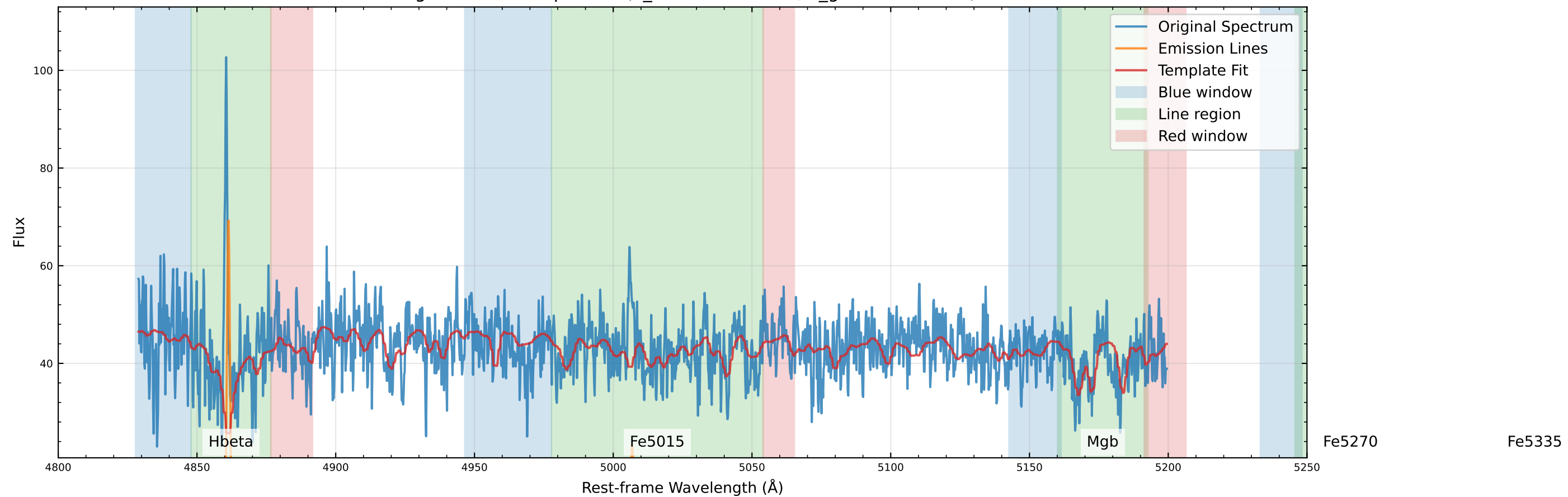
Original Data Comparison (v_star=-48.9 km/s, v_gas=-51.9 km/s)
