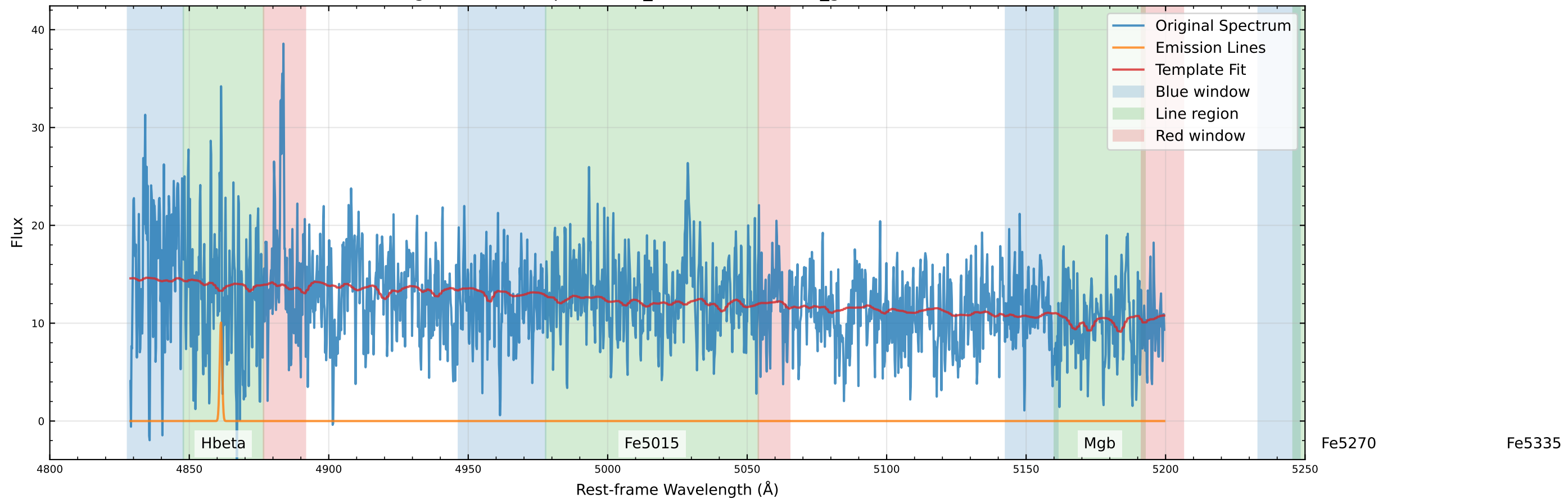
Original Data Comparison (v_star=-35.1 km/s, v_gas=-9.1 km/s)
