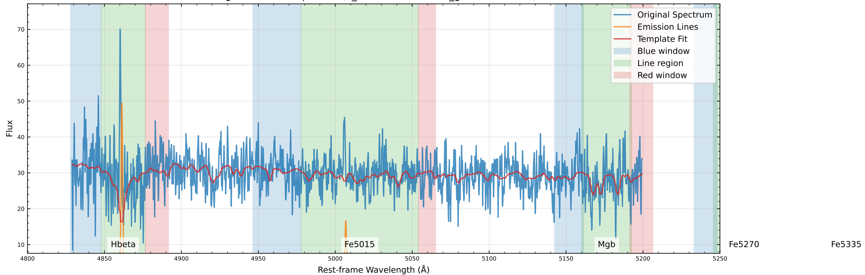
Original Data Comparison ( v_{\text{star}}=-56.4 km/s, v_{\text{gas}}=-60.6 km/s)
