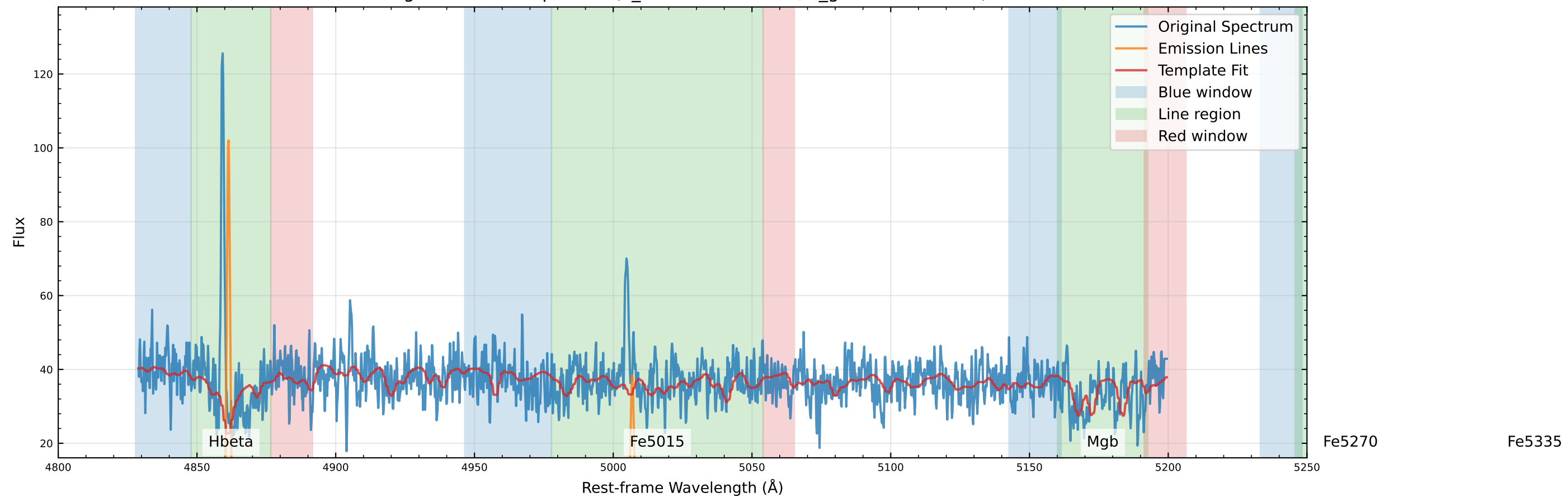
Original Data Comparison (v_star=-116.6 km/s, v_gas=-128.1 km/s)
