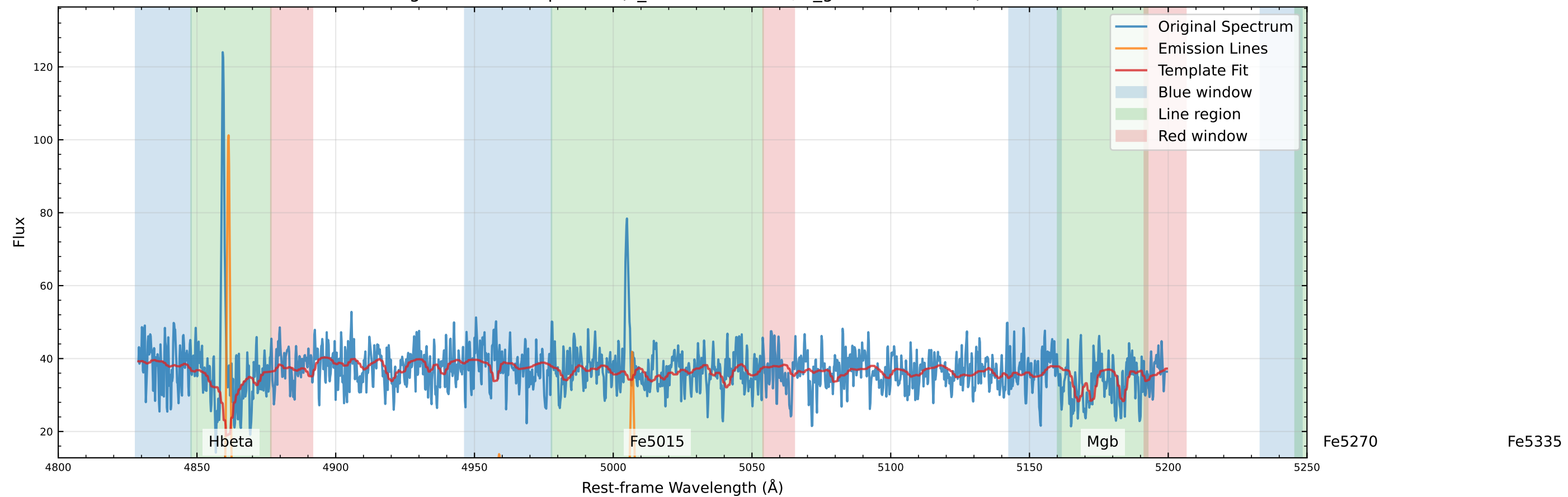
Original Data Comparison (v_star=-97.6 km/s, v_gas=-118.7 km/s)
