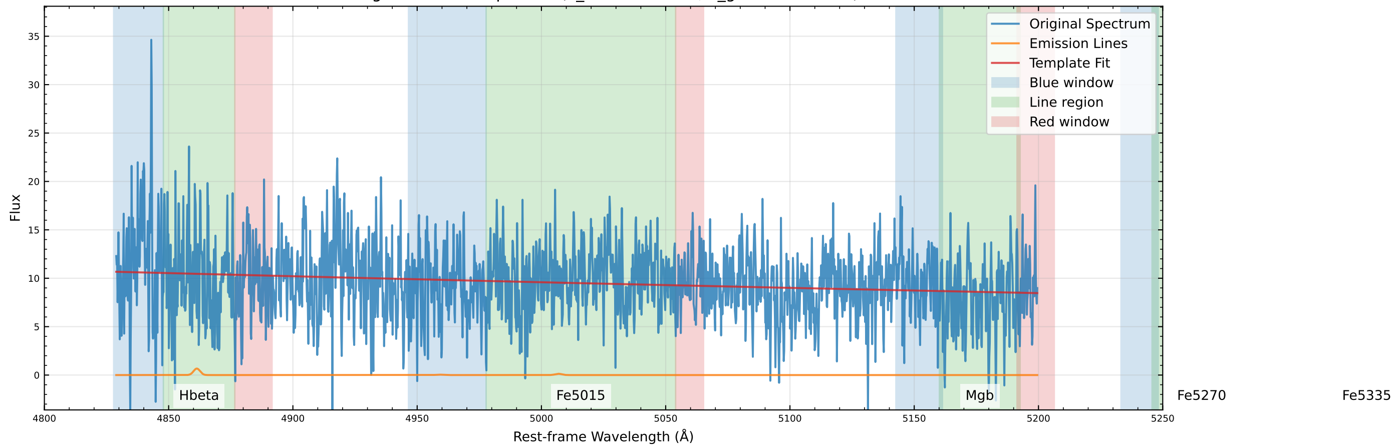
Original Data Comparison (v_star=0.0 km/s, v_gas=-16.9 km/s)
