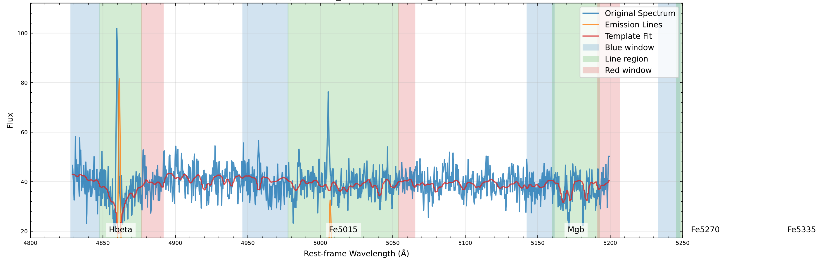
Original Data Comparison (v_star=-97.1 km/s, v_gas=-89.4 km/s)
