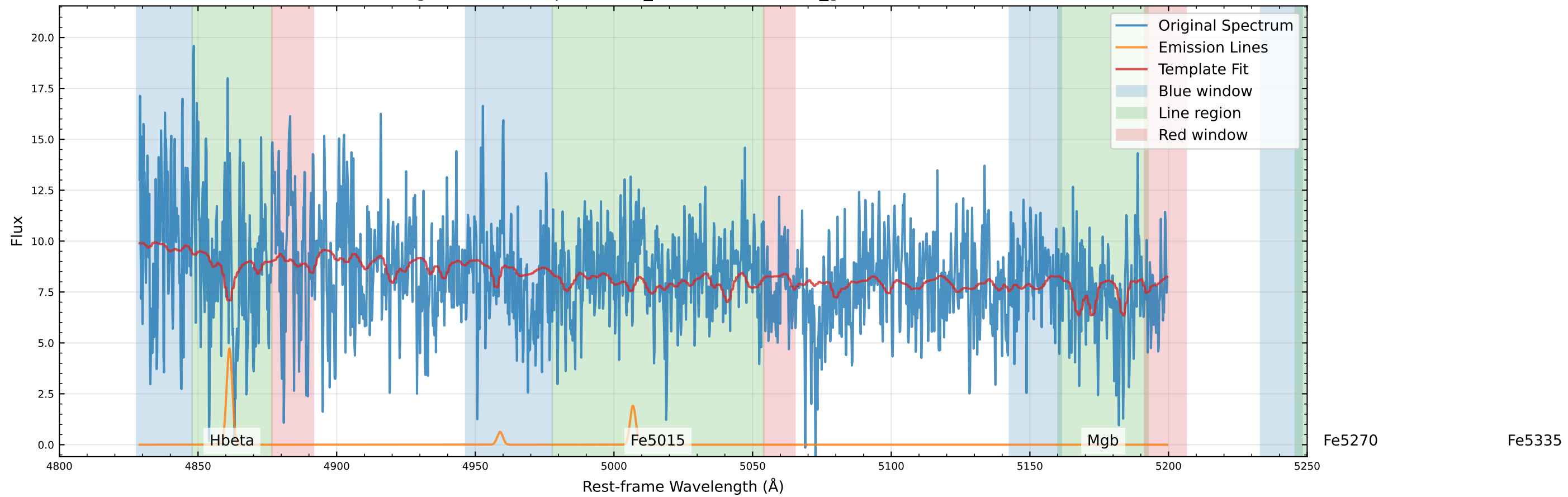
Original Data Comparison (v_star=-83.1 km/s, v_gas=-51.7 km/s)
