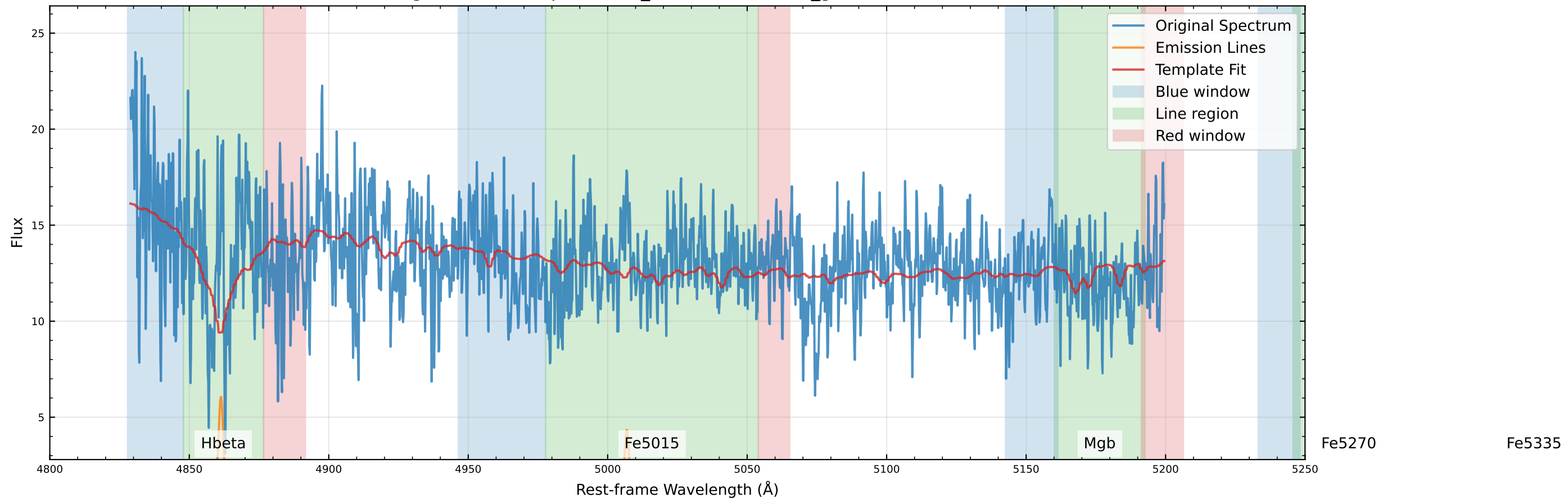
Original Data Comparison (v_star=12.0 km/s, v_gas=-19.6 km/s)
