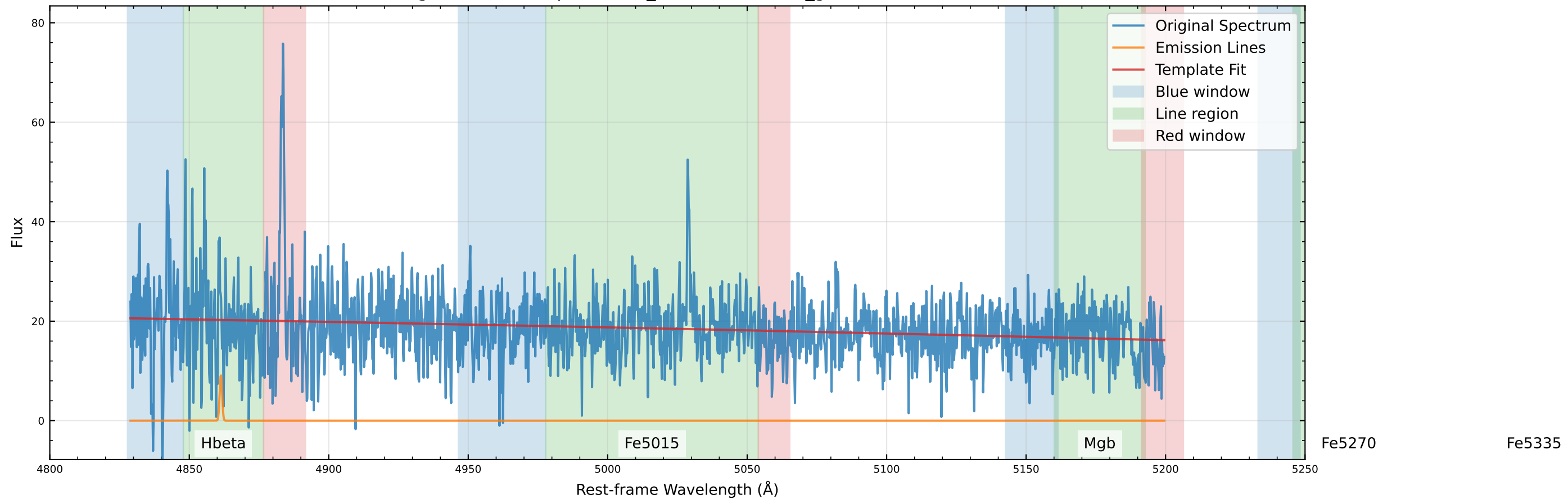
Original Data Comparison (v_star=0.0 km/s, v_gas=-26.5 km/s)
