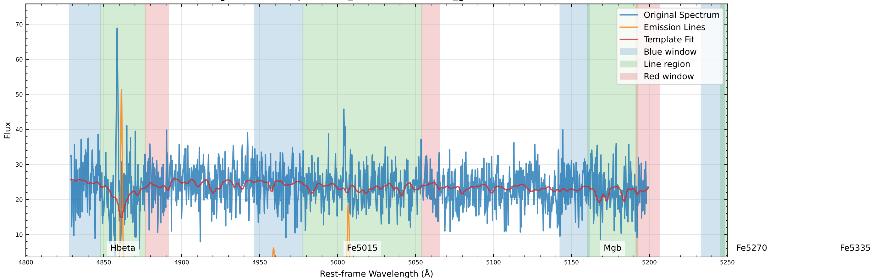
Original Data Comparison (v_star=-152.9 km/s, v_gas=-165.6 km/s)
