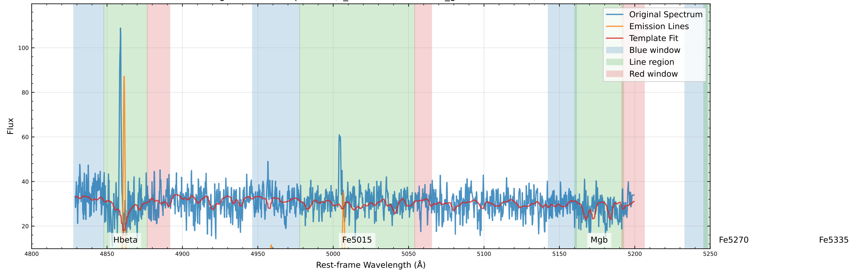
Original Data Comparison (v_star=-156.6 km/s, v_gas=-154.5 km/s)
