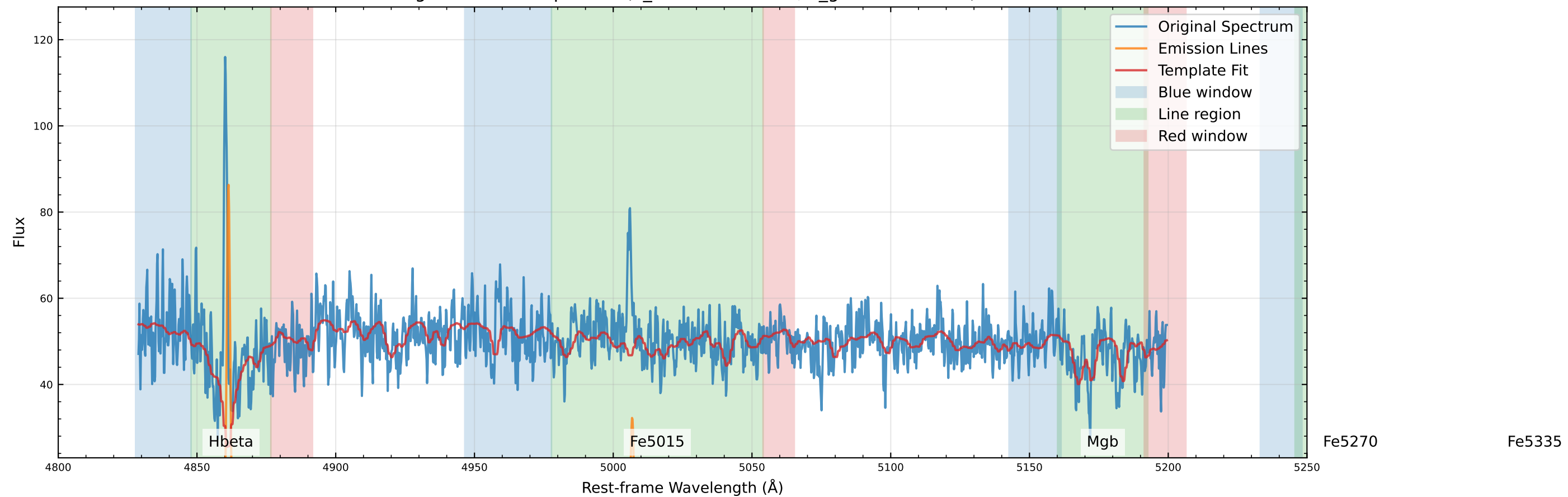
Original Data Comparison (v_star=-59.4 km/s, v_gas=-64.9 km/s)
