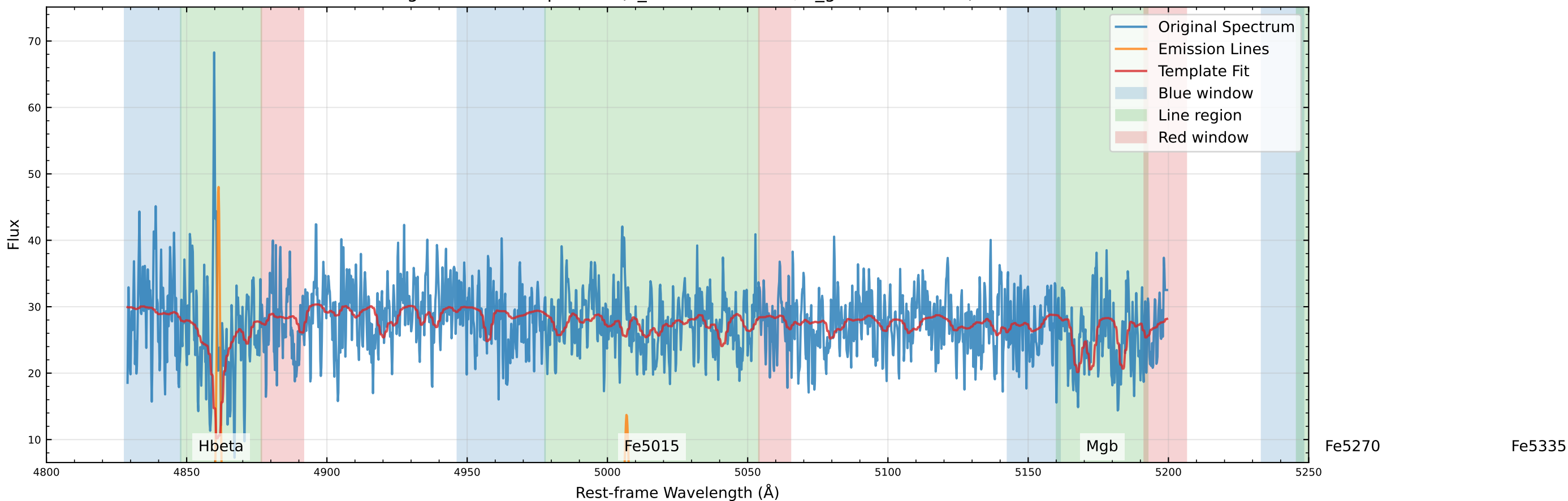
Original Data Comparison (v_star=-96.3 km/s, v_gas=-85.1 km/s)
