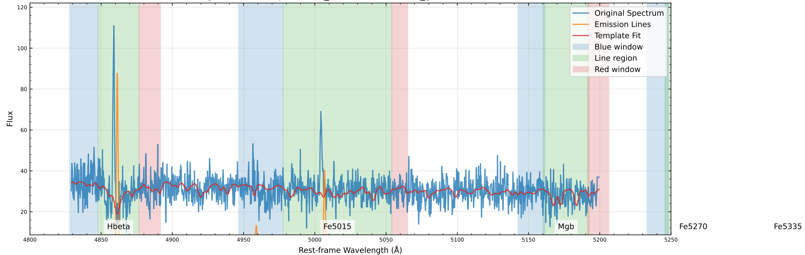
Original Data Comparison (v_star=-153.7 km/s, v_gas=-153.1 km/s)
