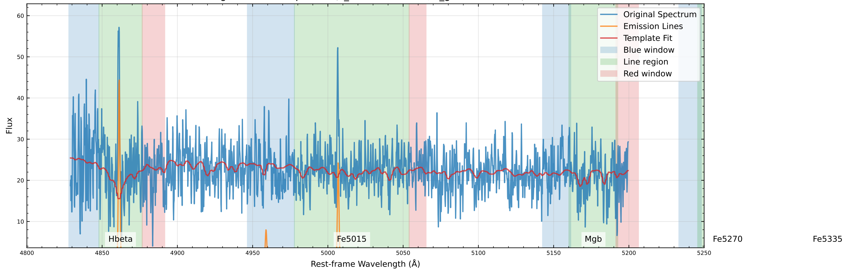
Original Data Comparison (v_star=-14.0 km/s, v_gas=-18.4 km/s)
