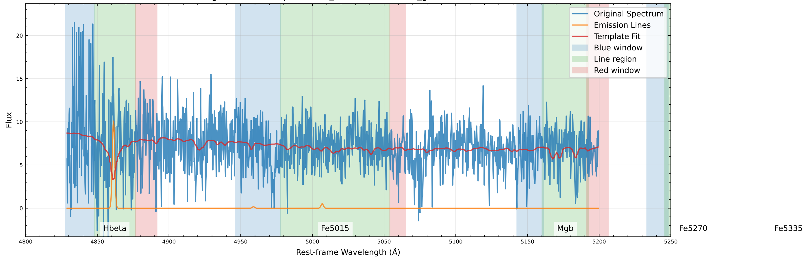
Original Data Comparison (v_star=19.1 km/s, v_gas=-20.1 km/s)
