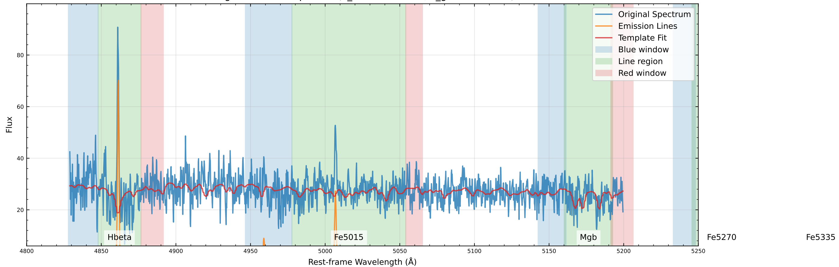
Original Data Comparison (v_star=-8.0 km/s, v_gas=-8.1 km/s)
