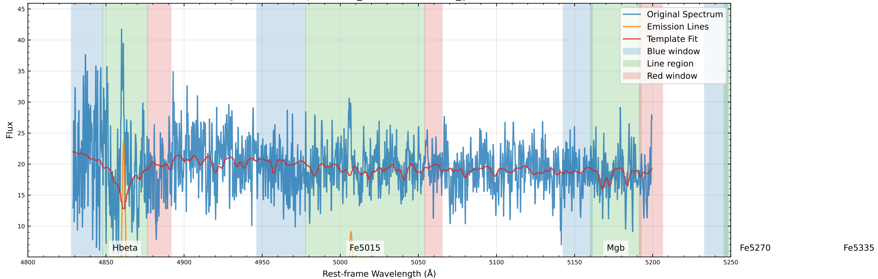
Original Data Comparison (v_star=-74.3 km/s, v_gas=-56.1 km/s)
