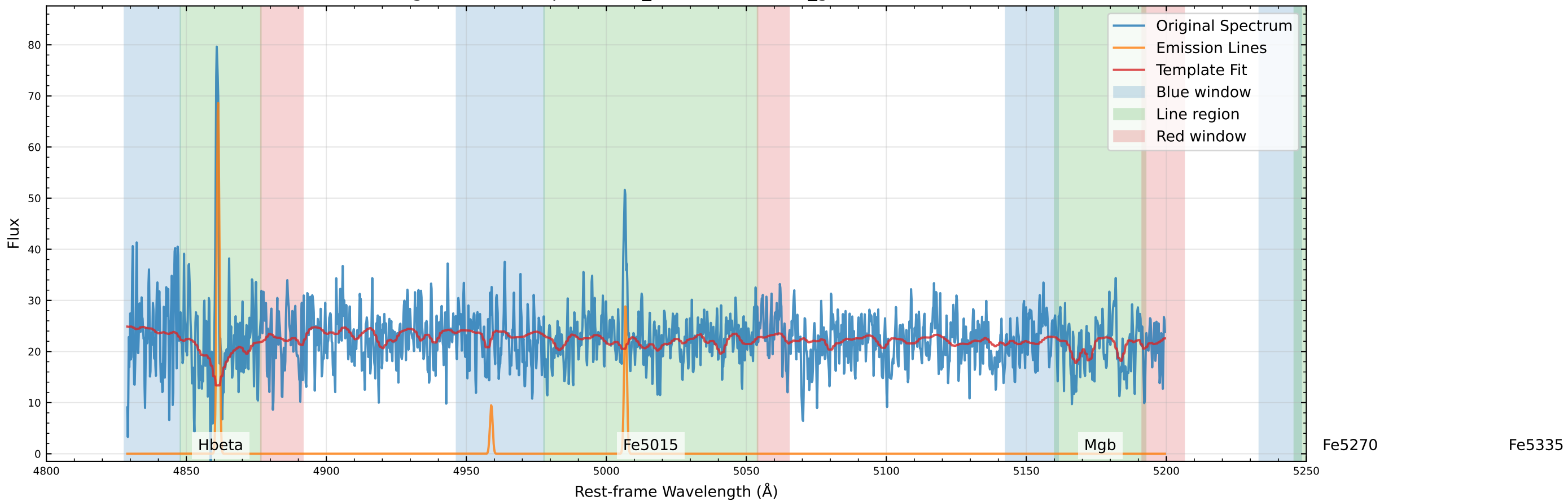
Original Data Comparison (v_star=-9.8 km/s, v_gas=-20.1 km/s)
