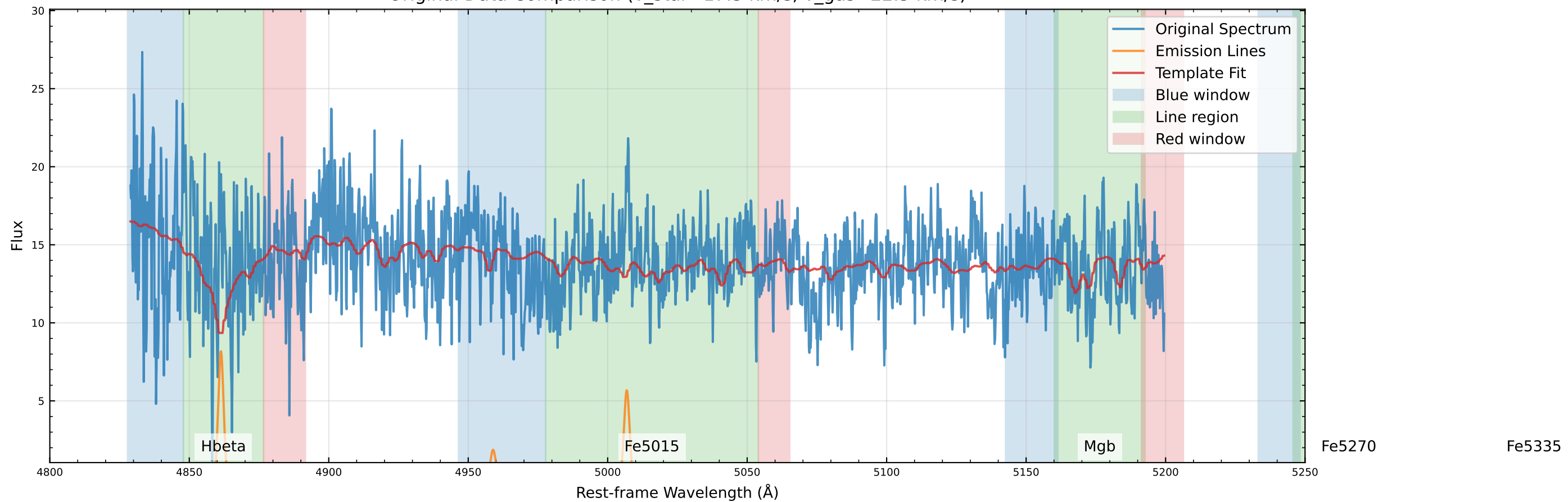
Original Data Comparison (v_star=17.3 km/s, v_gas=22.5 km/s)
