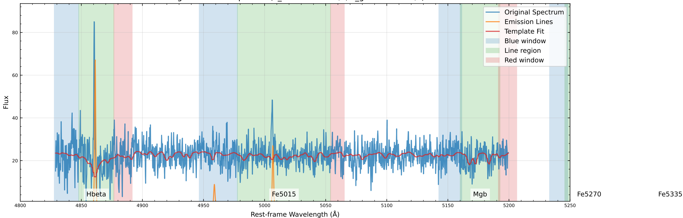
Original Data Comparison (v_star=-70.1 km/s, v_gas=-47.0 km/s)
