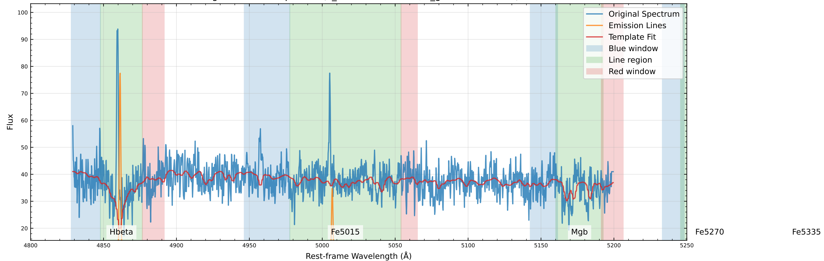
Original Data Comparison (v_star=-135.6 km/s, v_gas=-109.6 km/s)
