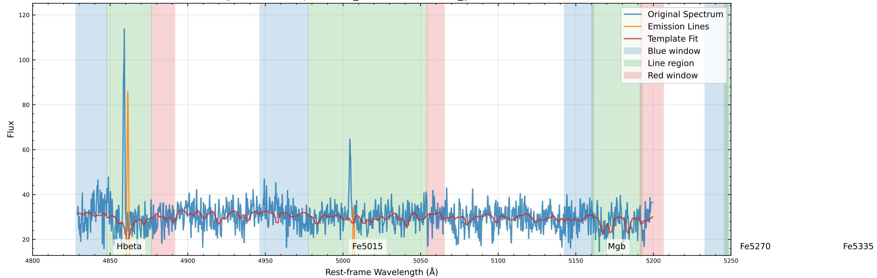
Original Data Comparison (v_star=-144.0 km/s, v_gas=-148.1 km/s)
