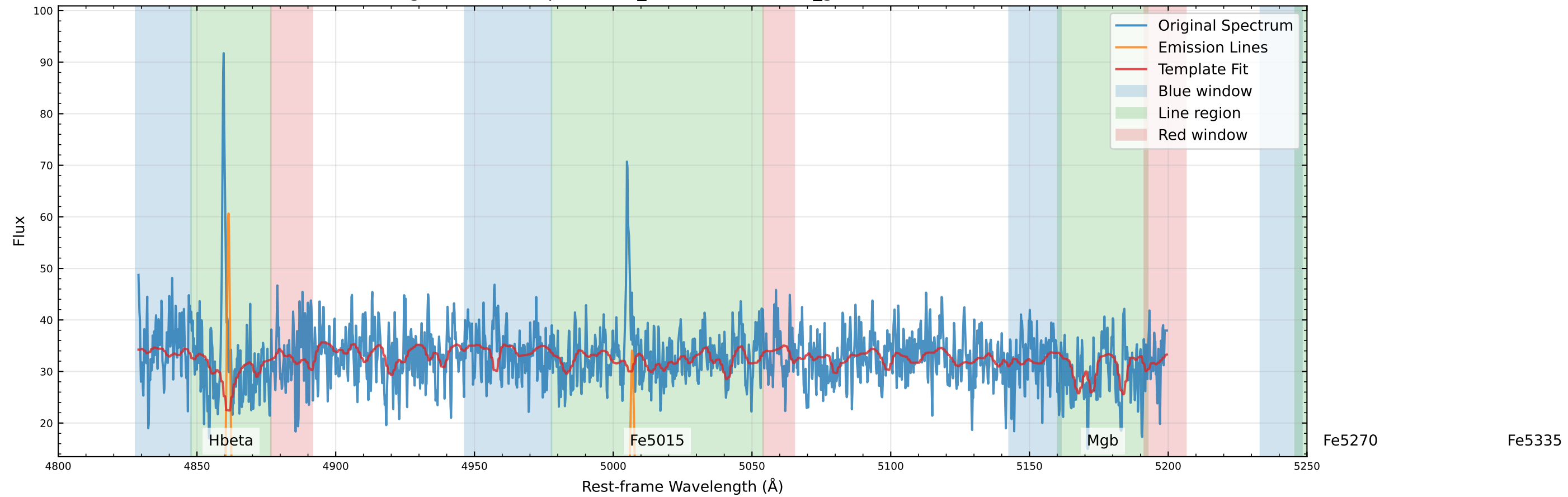
Original Data Comparison (v_star=-93.4 km/s, v_gas=-103.3 km/s)
