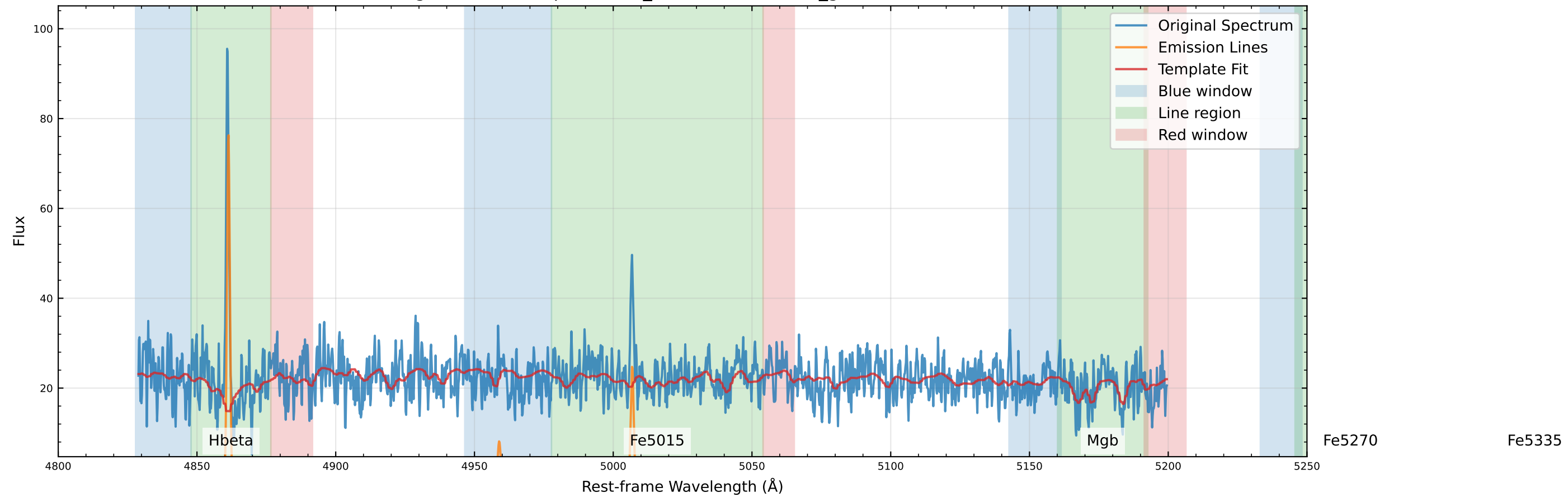
Original Data Comparison (v_star=-28.0 km/s, v_gas=-19.9 km/s)
