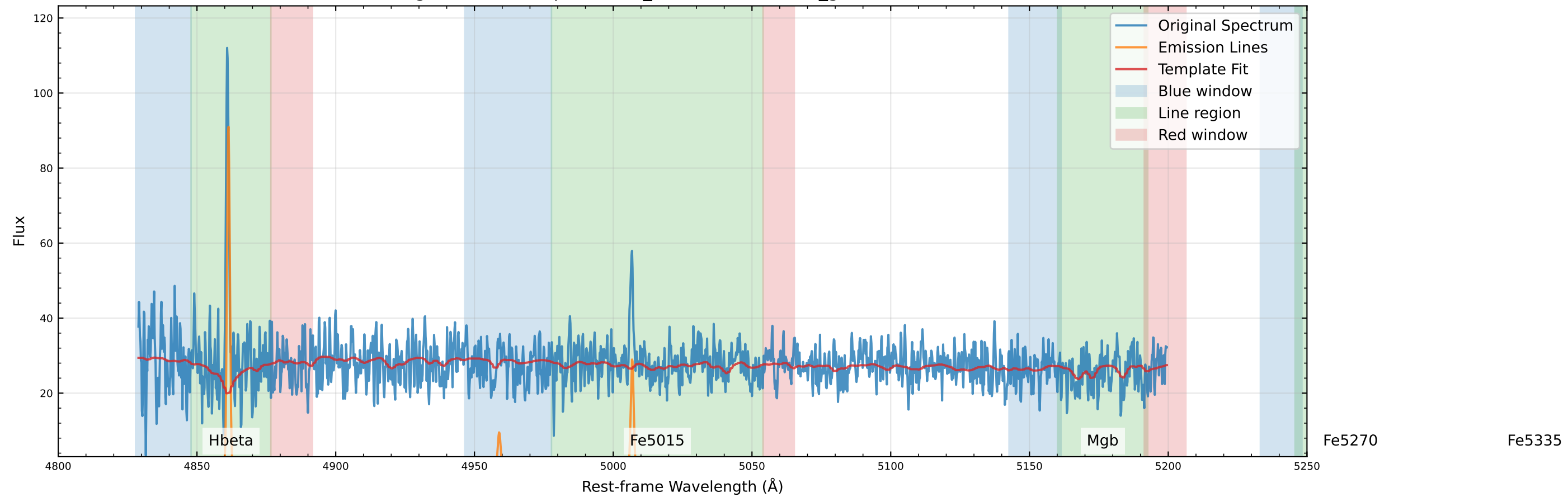
Original Data Comparison (v_star=-40.9 km/s, v_gas=-21.6 km/s)
