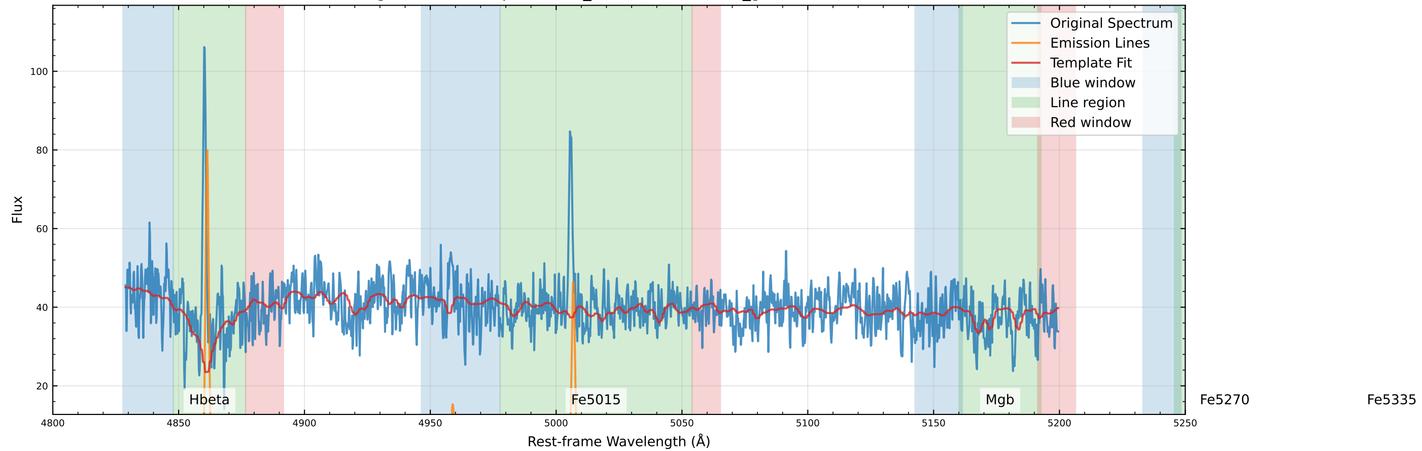
Original Data Comparison (v_star=-77.5 km/s, v_gas=-66.8 km/s)
