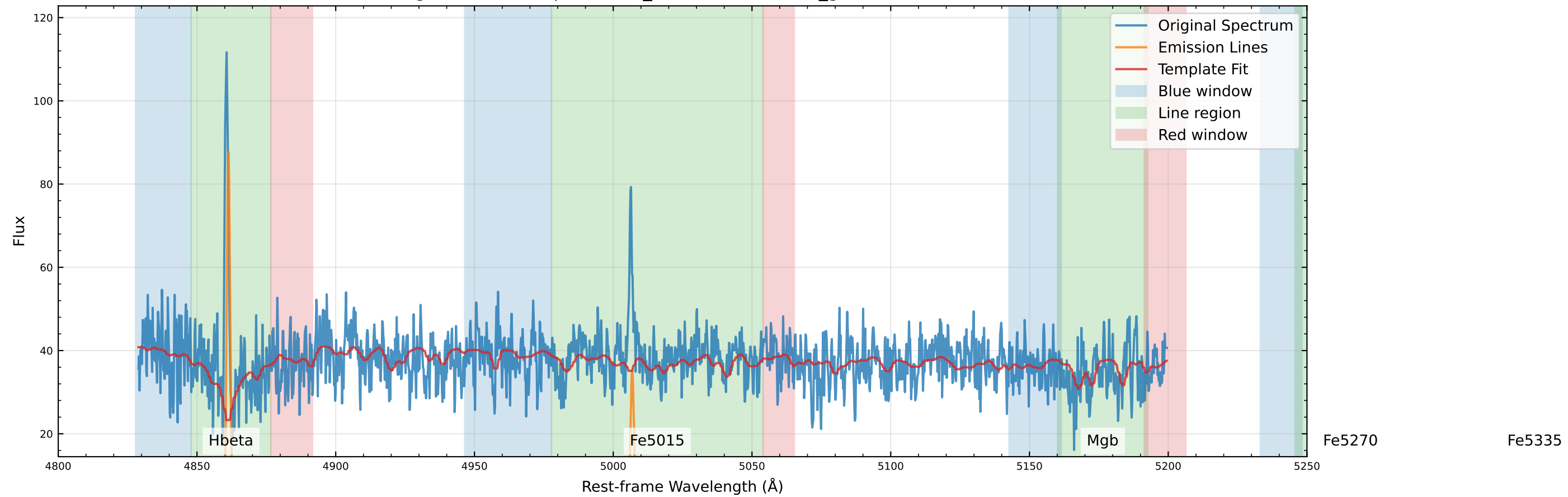
Original Data Comparison (v_star=-68.0 km/s, v_gas=-40.5 km/s)
