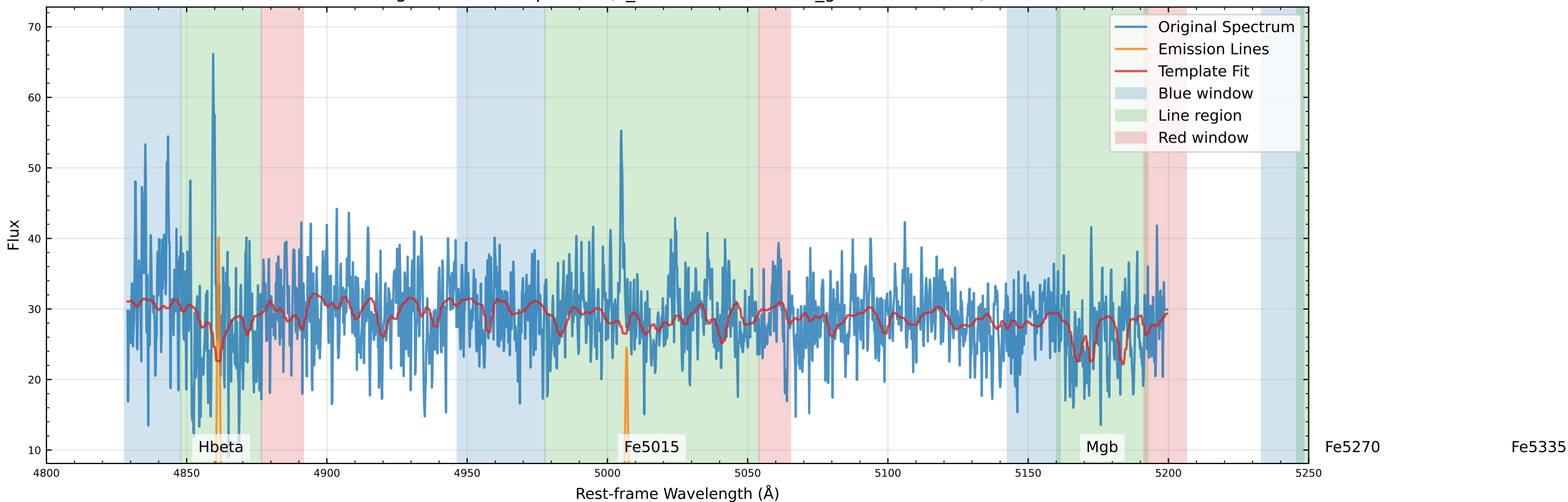
Original Data Comparison (v_star=-113.2 km/s, v_gas=-104.9 km/s)
