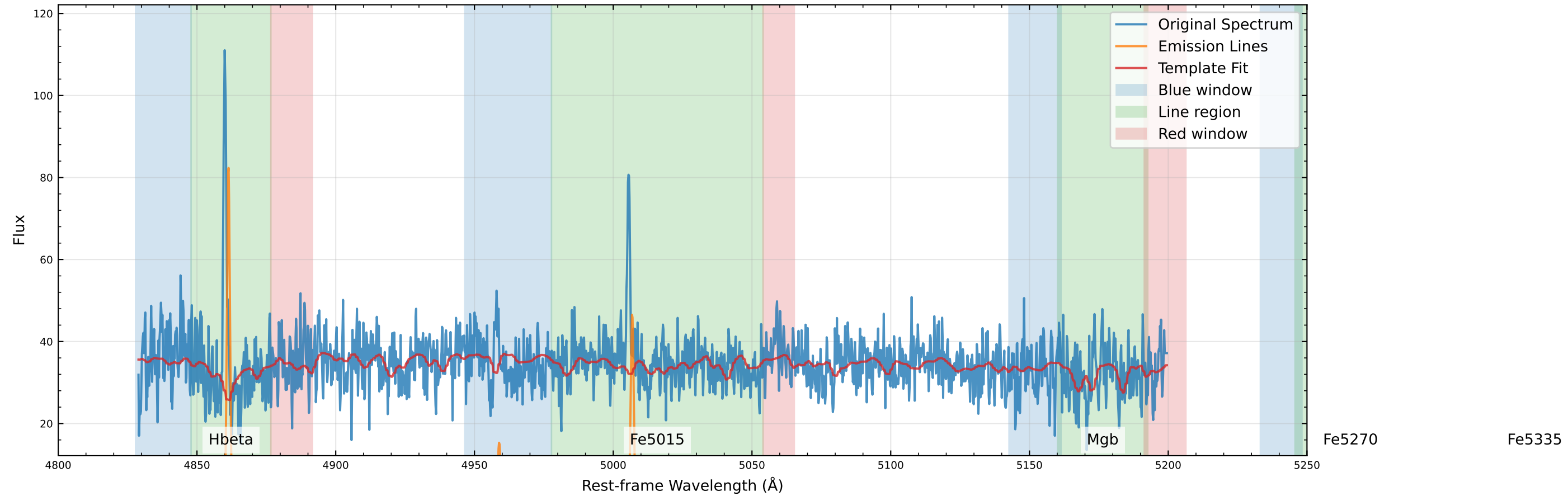
Original Data Comparison (v_star=-87.5 km/s, v_gas=-78.8 km/s)
