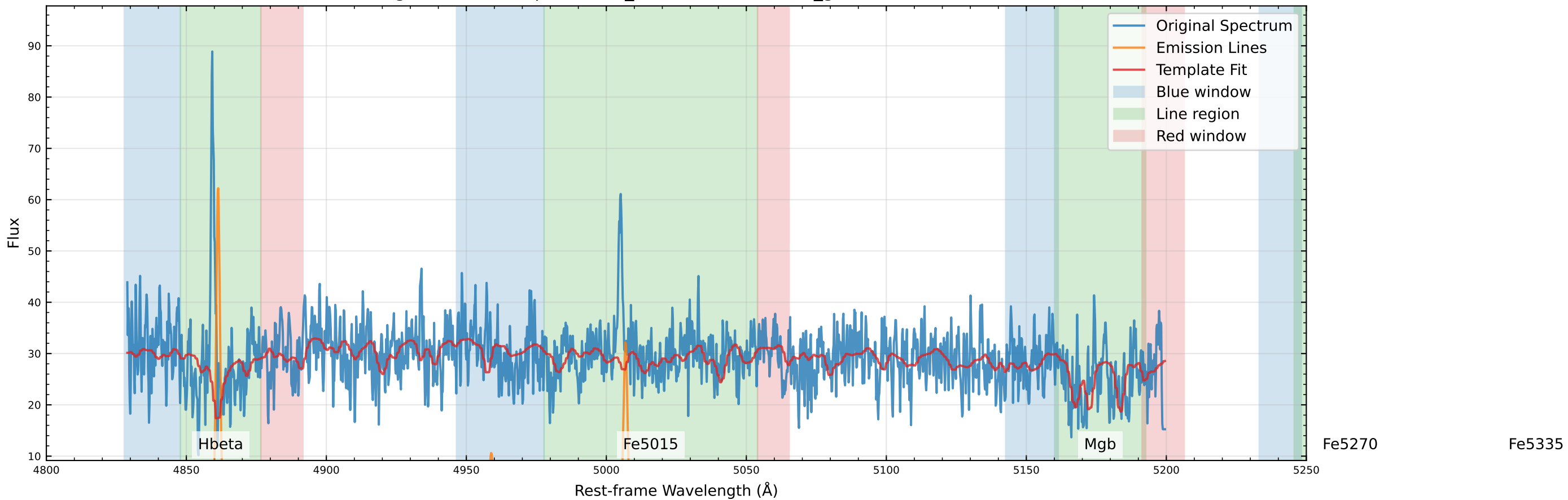
Original Data Comparison (v_star=-104.2 km/s, v_gas=-117.9 km/s)
