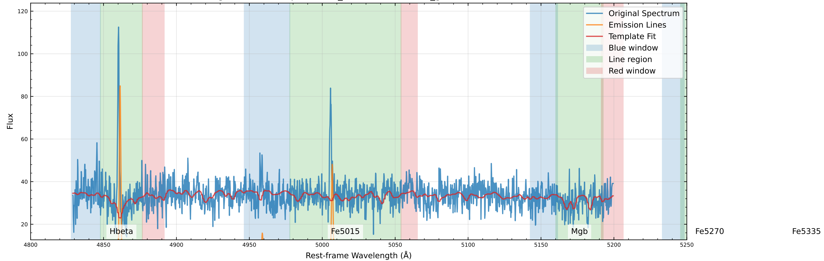
Original Data Comparison (v_star=-69.6 km/s, v_gas=-68.5 km/s)
