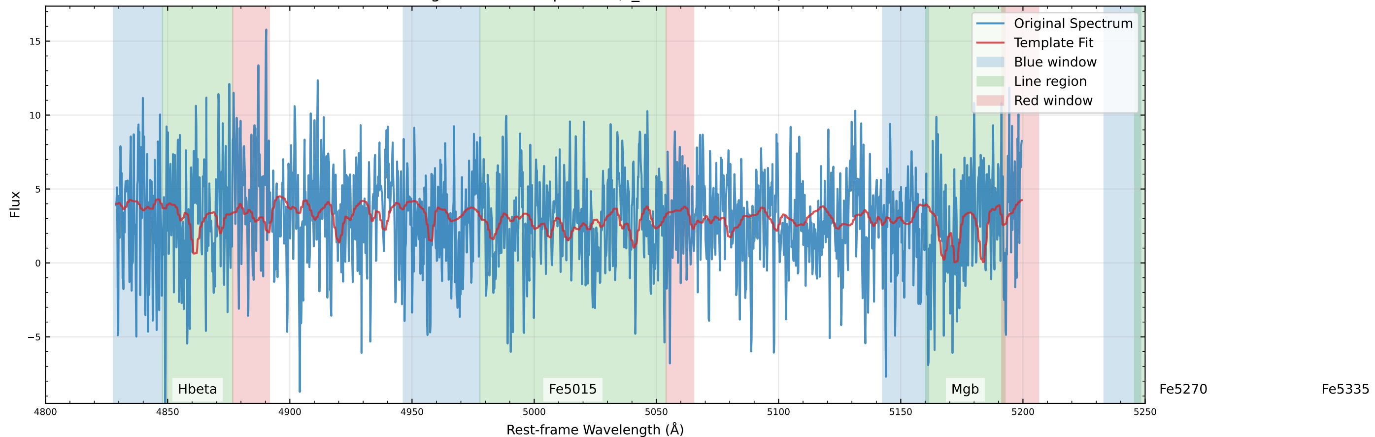
Original Data Comparison (v_star=-856.3 km/s)
