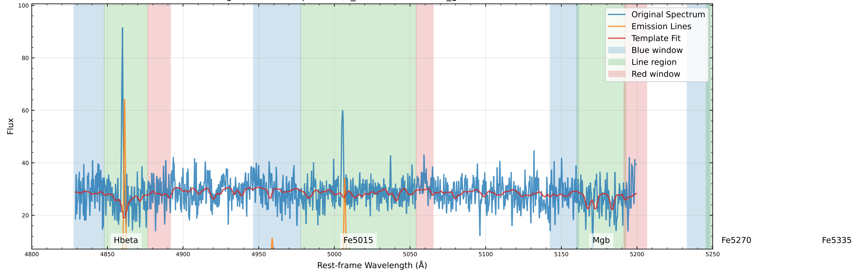
Original Data Comparison (v_star=-96.8 km/s, v_gas=-89.5 km/s)
