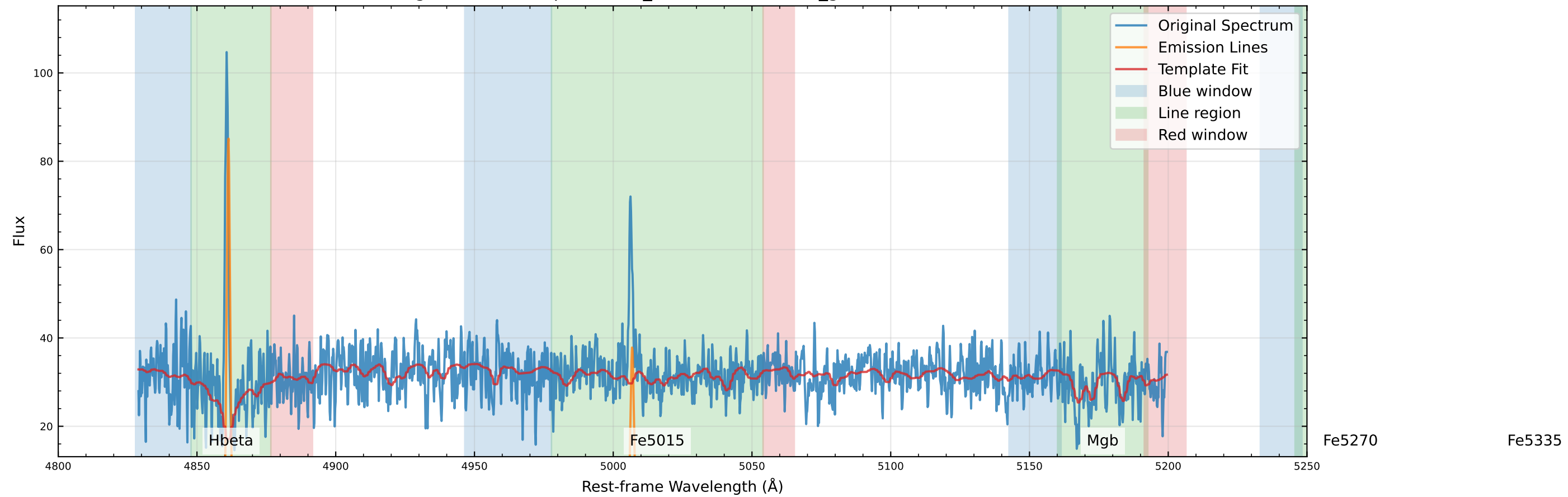
Original Data Comparison (v_star=-57.7 km/s, v_gas=-37.7 km/s)
