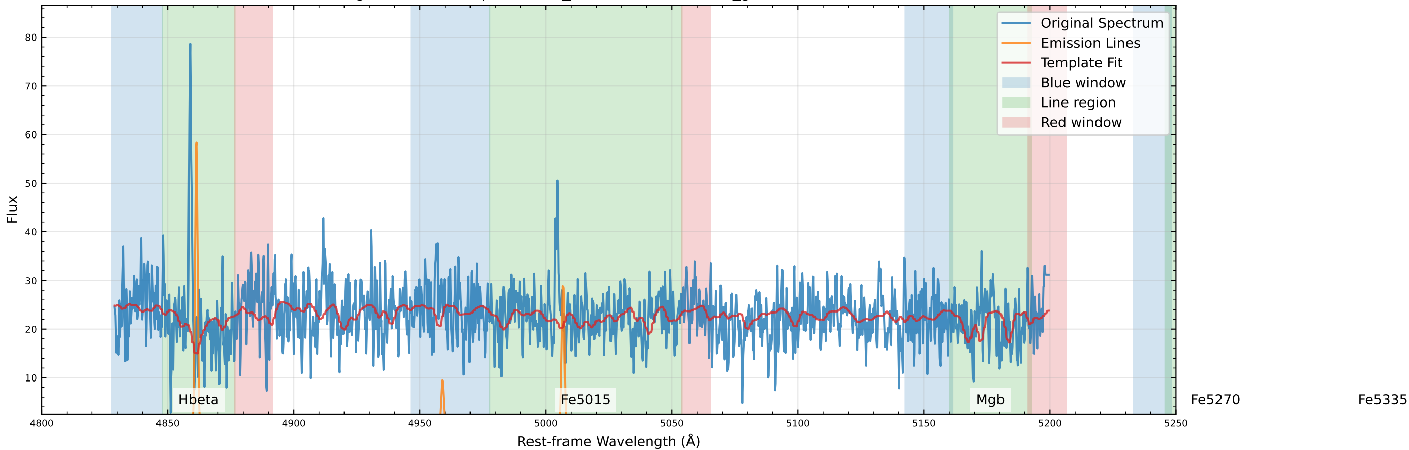
Original Data Comparison (v_star=-140.5 km/s, v_gas=-147.9 km/s)
