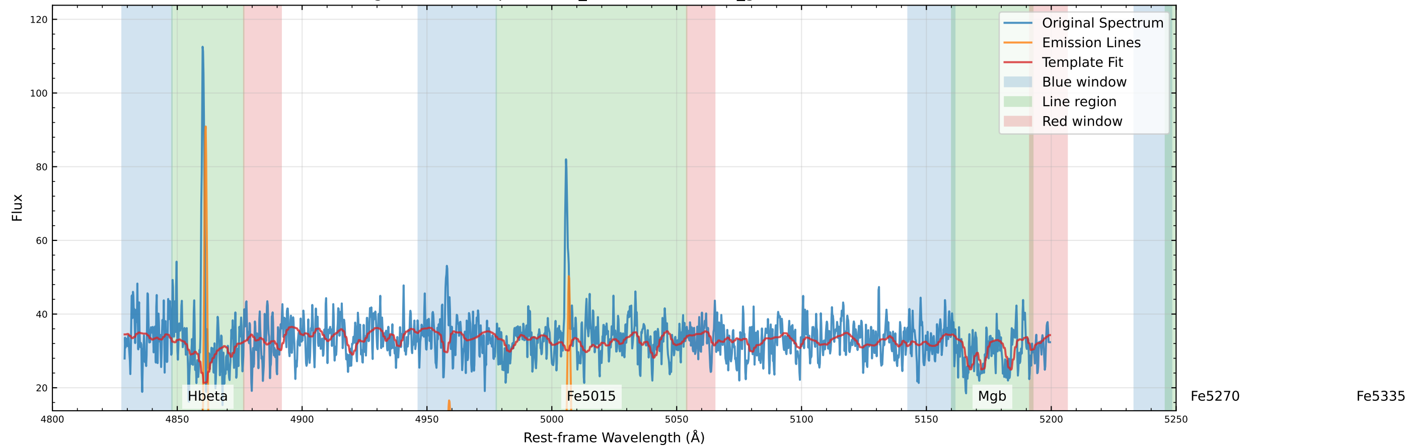
Original Data Comparison (v_star=-76.3 km/s, v_gas=-63.9 km/s)
