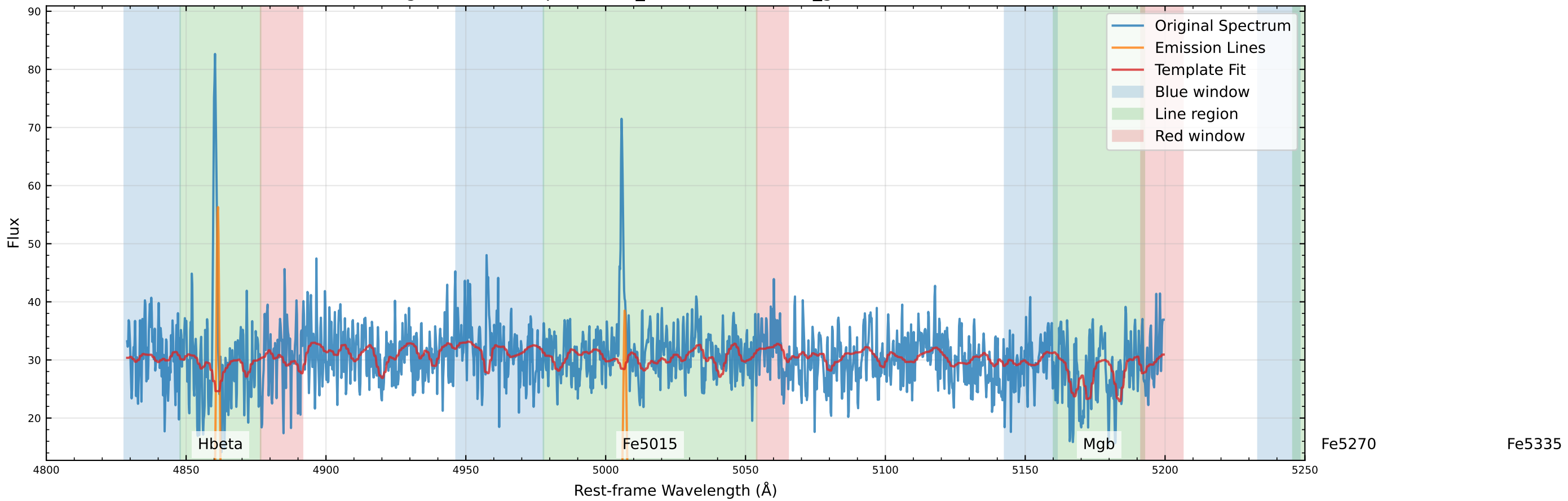
Original Data Comparison (v_star=-60.8 km/s, v_gas=-63.1 km/s)
