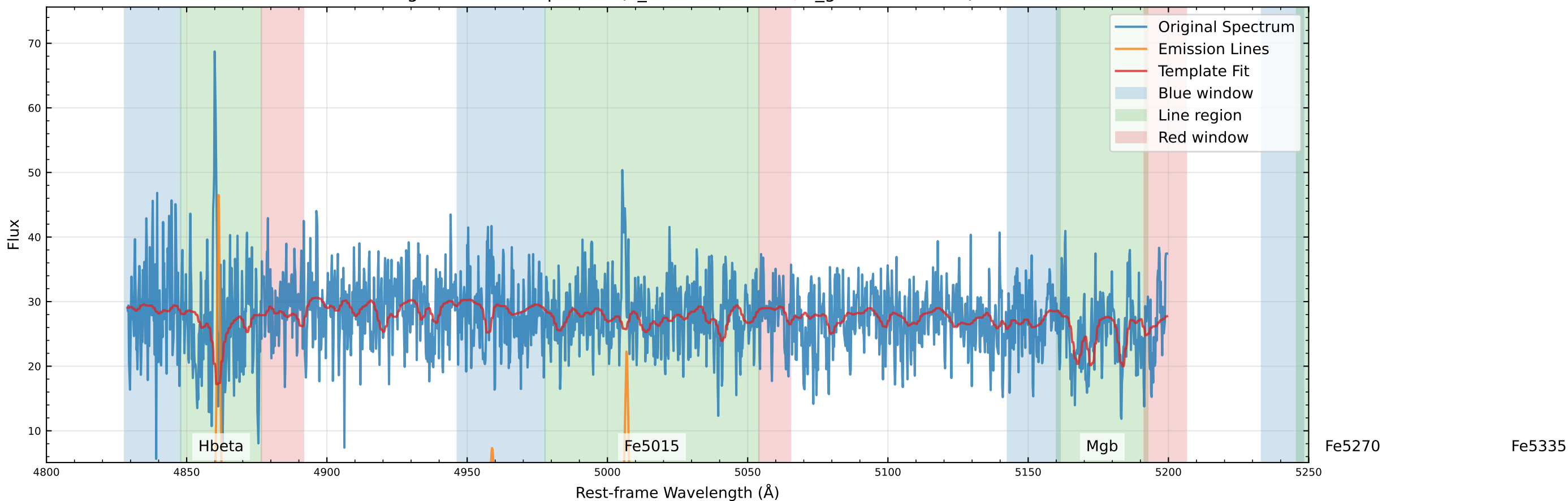
Original Data Comparison (v_star=-63.4 km/s, v_gas=-75.5 km/s)
