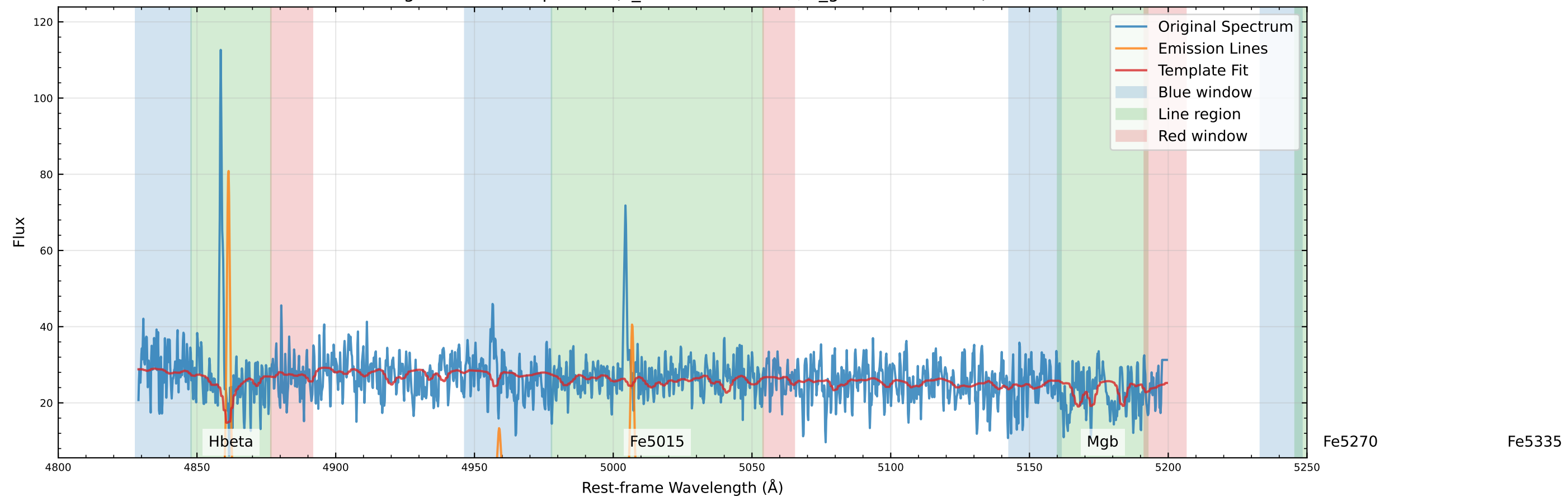
Original Data Comparison (v_star=-199.1 km/s, v_gas=-160.9 km/s)
