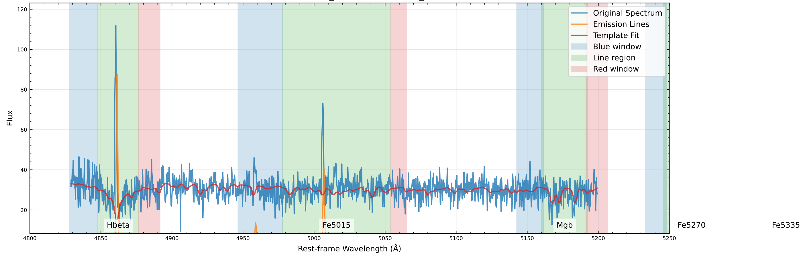
Original Data Comparison (v_star=-58.7 km/s, v_gas=-53.9 km/s)
