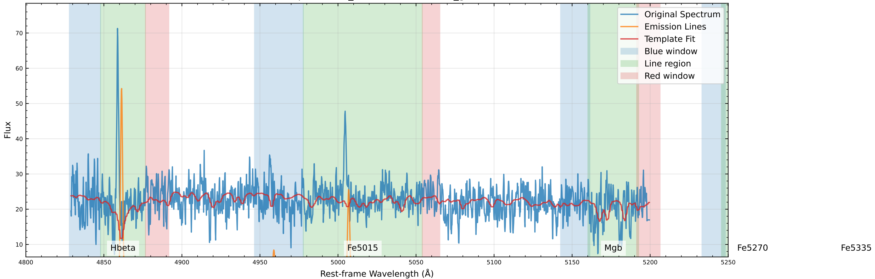
Original Data Comparison (v_star=-166.5 km/s, v_gas=-151.7 km/s)
