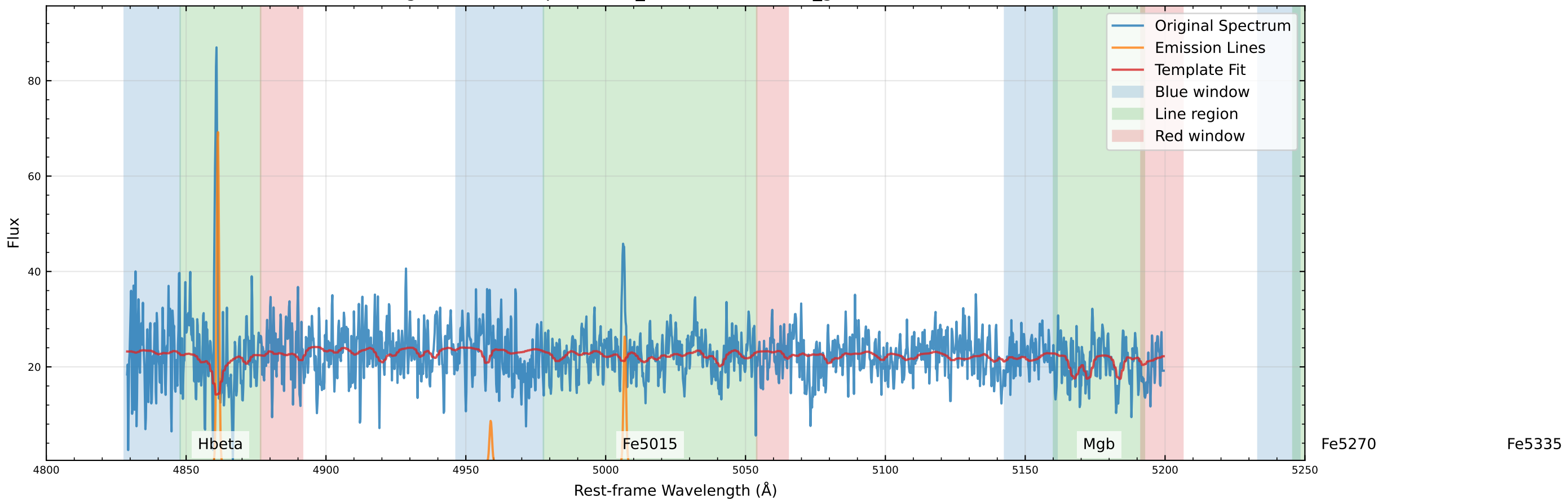
Original Data Comparison (v_star=-56.9 km/s, v_gas=-37.1 km/s)
