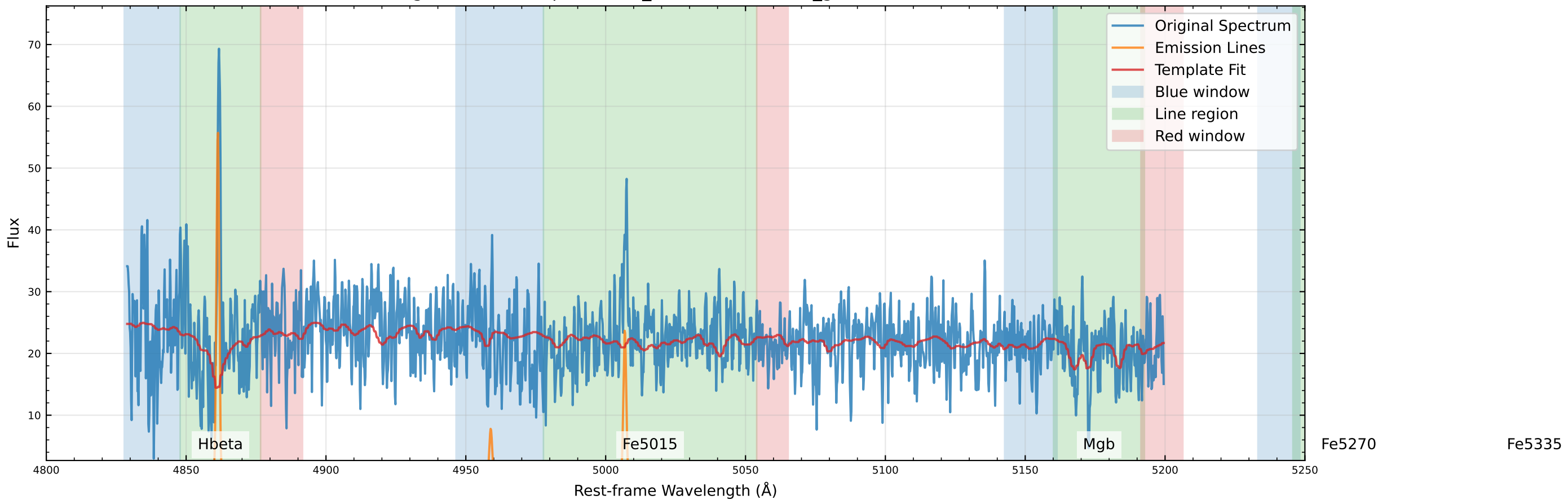
Original Data Comparison ( v_{\text{star}}=44.6 km/s, v_{\text{gas}}=24.8 km/s)
