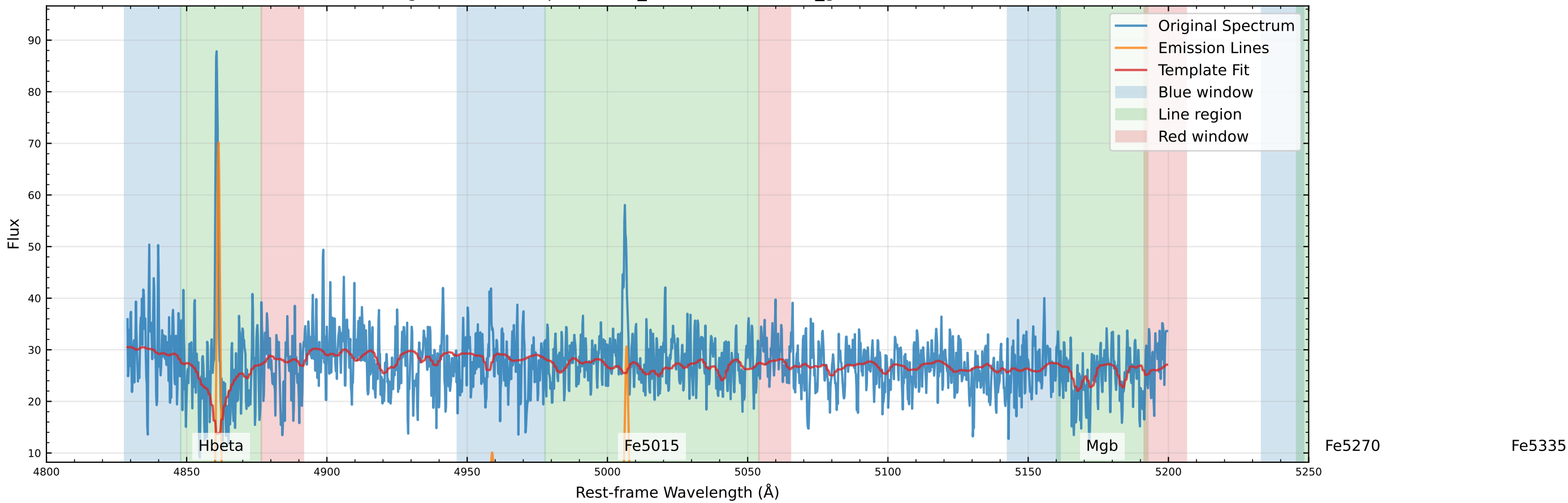
Original Data Comparison (v_star=-58.7 km/s, v_gas=-38.3 km/s)
