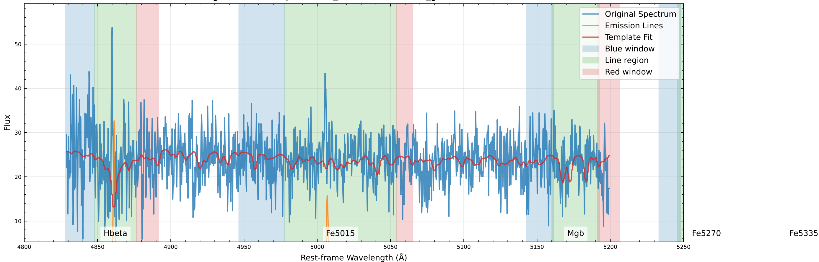
Original Data Comparison (v_star=-92.7 km/s, v_gas=-87.0 km/s)
