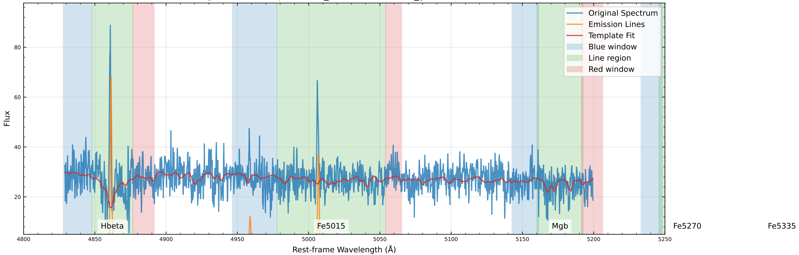
Original Data Comparison (v_star=-20.2 km/s, v_gas=-35.6 km/s)
