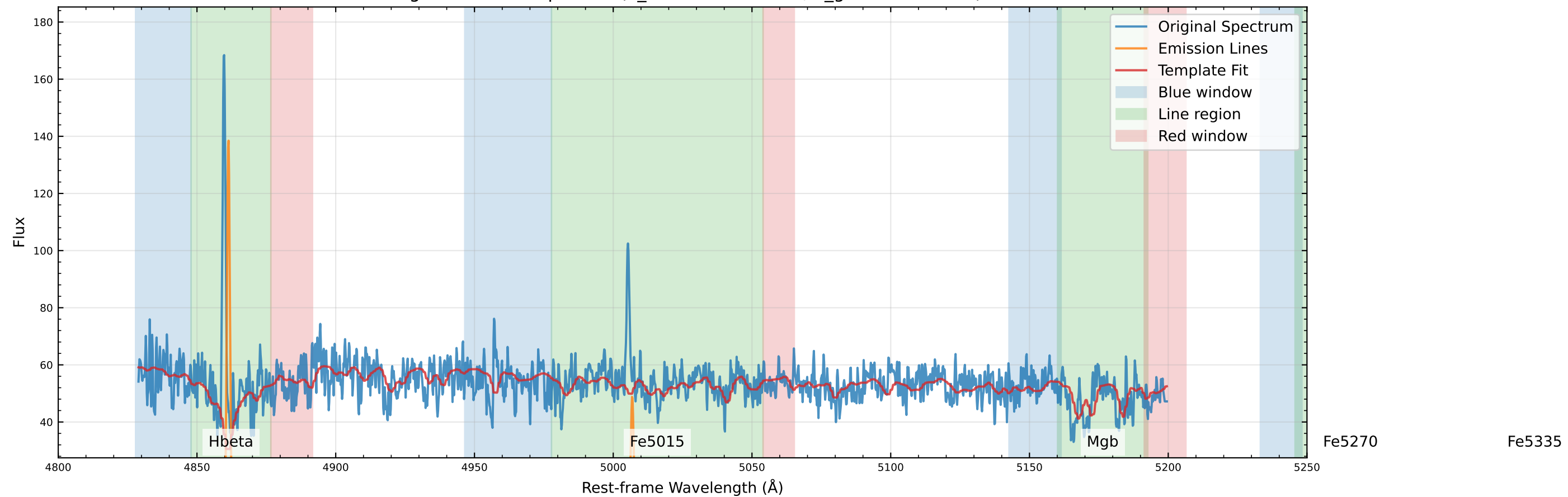
Original Data Comparison (v_star=-100.3 km/s, v_gas=-96.6 km/s)
